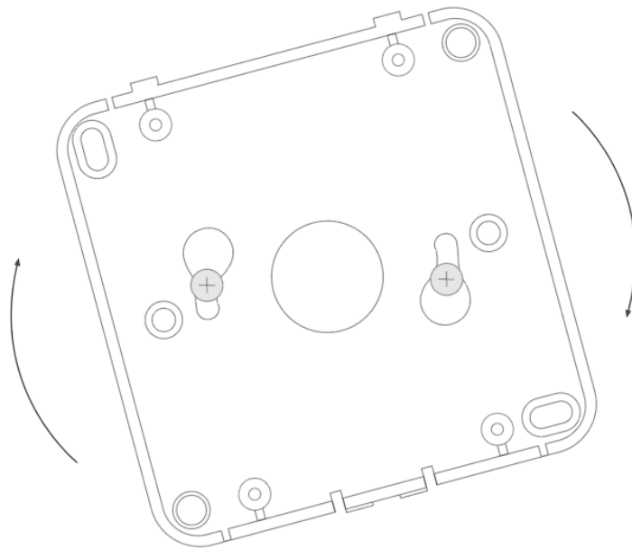
Figure 3 Mounting the device using two screws at an angle.
