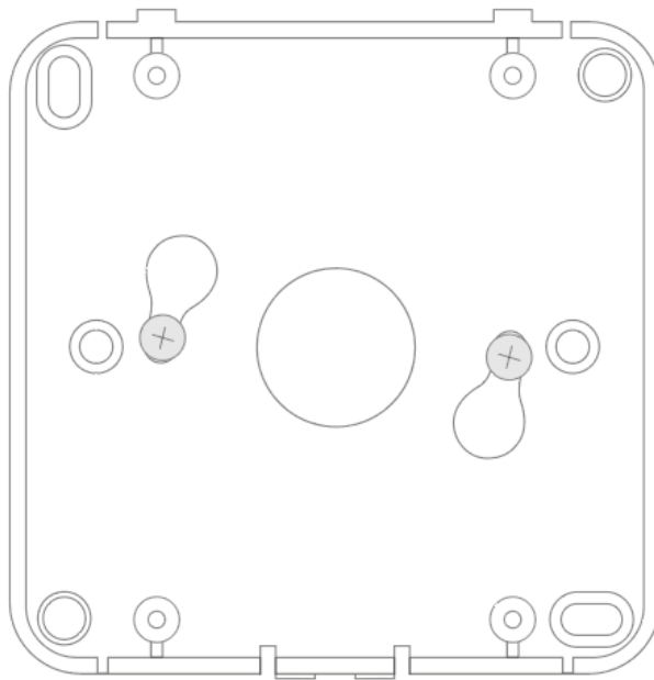
Figure 3 Mounting the device using two screws at an angle.
